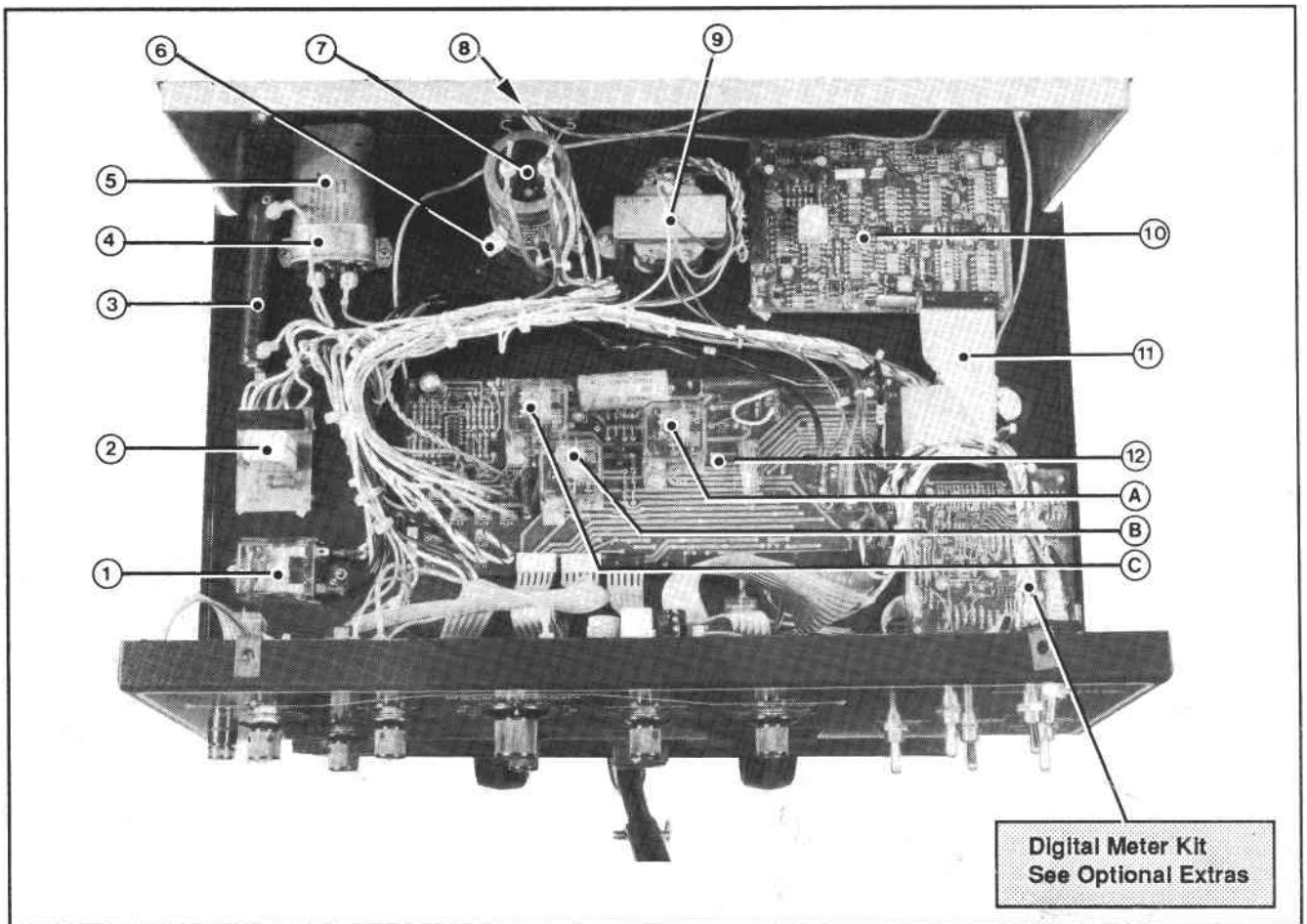
Fig. B - Top compartment components
