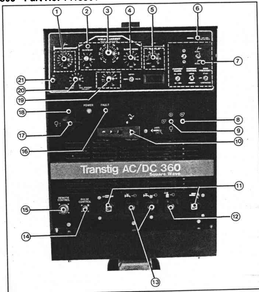
Fig. A. - Front View Components
