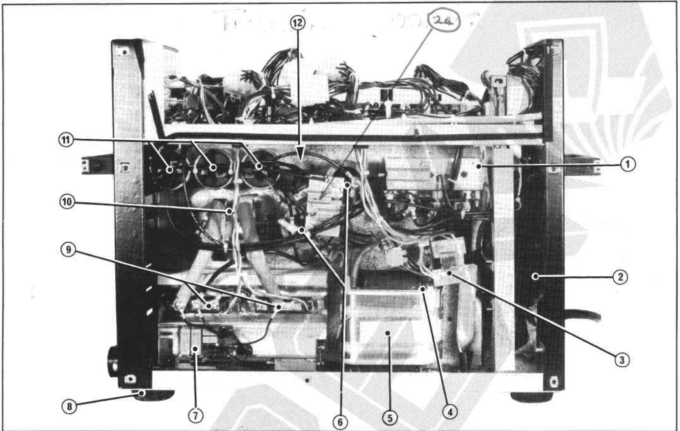
Fig. B - Right hand side view
