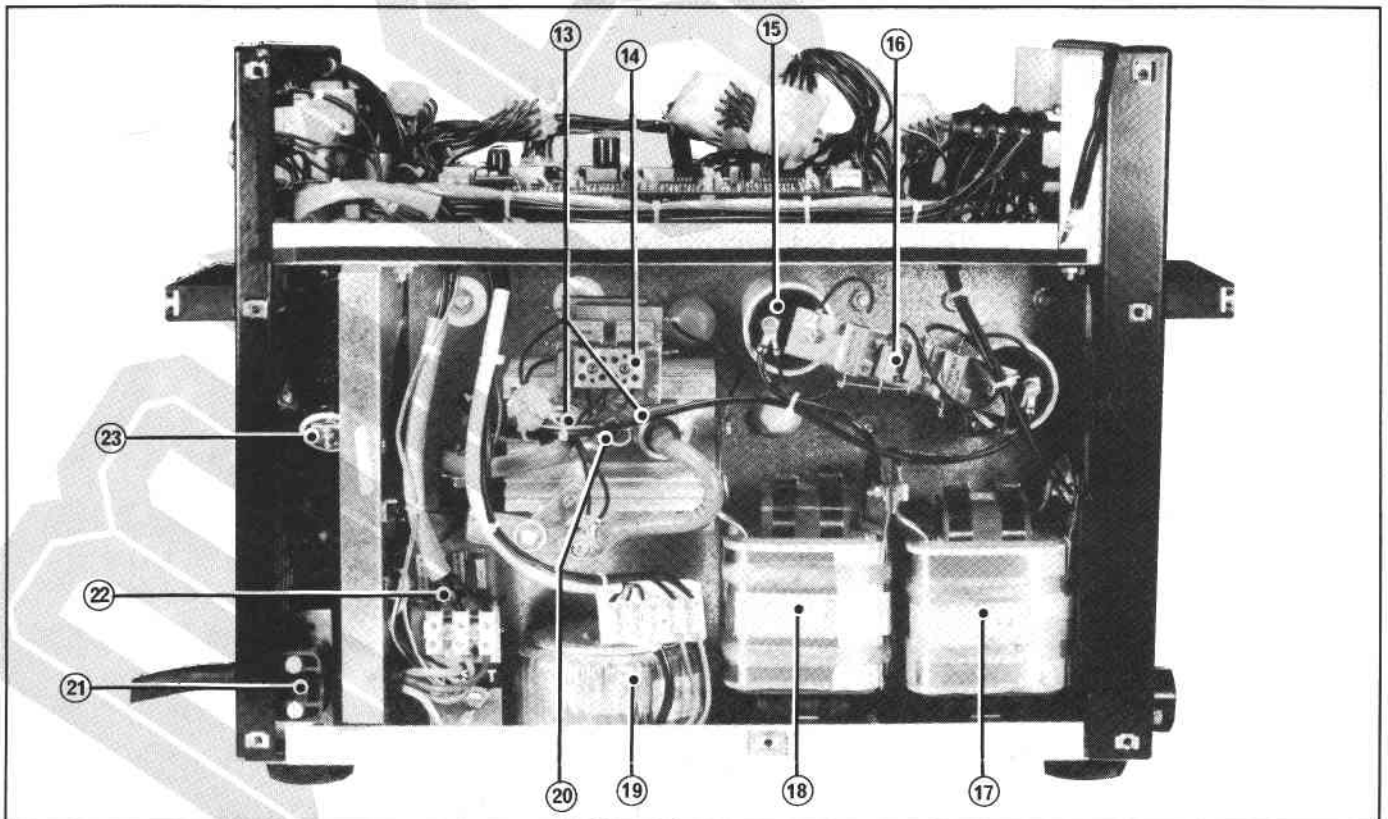
Fig. C - Left hand side view
